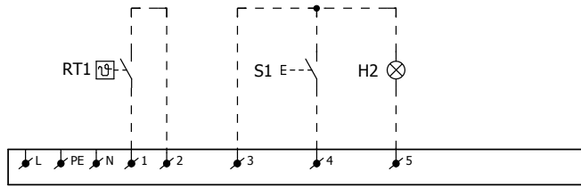
External connections
