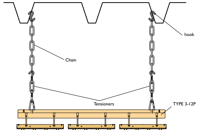
Method F Suspension by means of chains and tensioners
