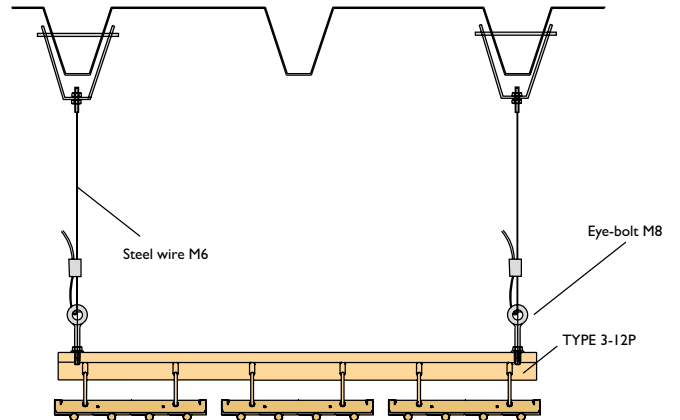
Method D Suspension by means of hangers
