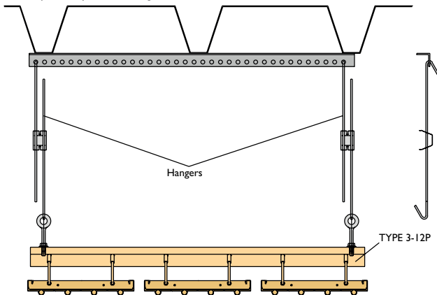
Method C Suspension by means of hangers
