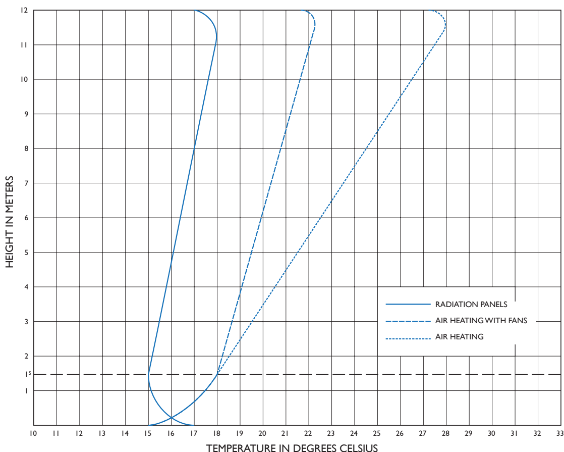
CHART (the difference in the vertical temperature gradient for radiation heating and air-heating)
