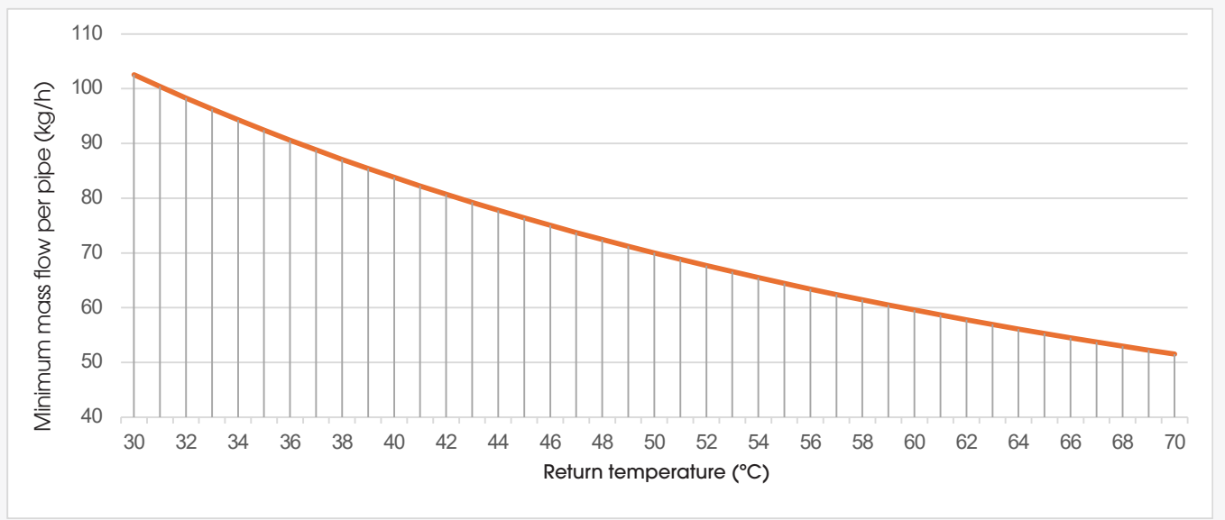
Graph 4.3 Minimum mass flow required per return temperature.
